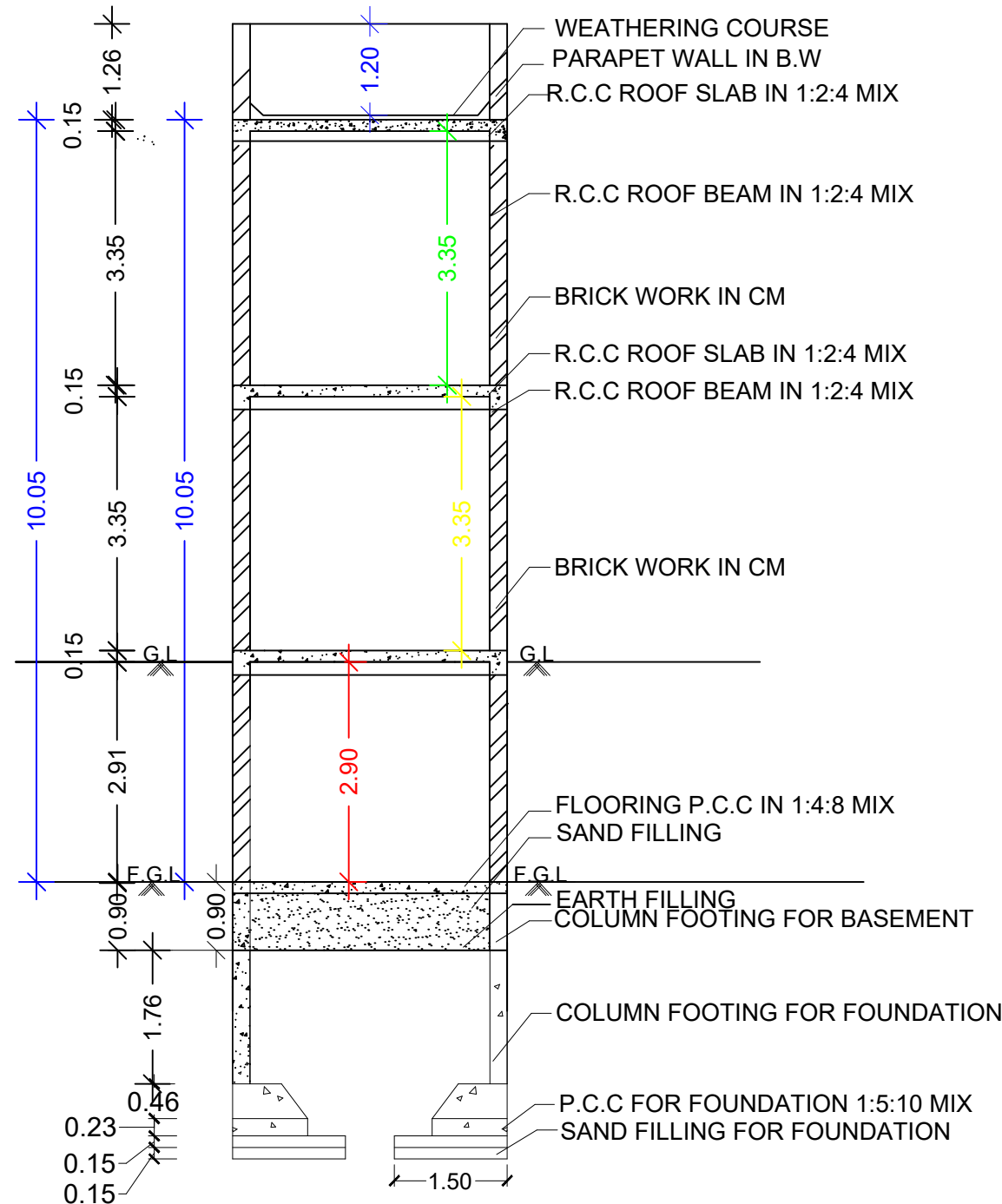
SECTION ON-AA
