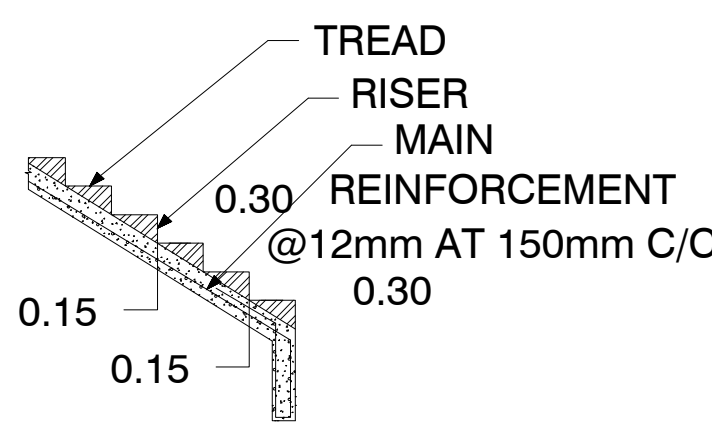
STAIRCASE DETAILES
