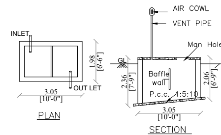
SEPTIC TANK
