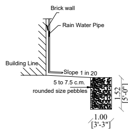
PERCOLATION PIT
