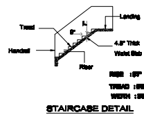
STAIRCASE DETAIL
