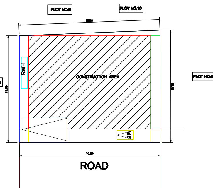
SITE PLAN
