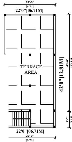
TERRACE FLOOR
