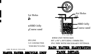
RAIN WATER HARVESTING UNIT TANK DETAIL
