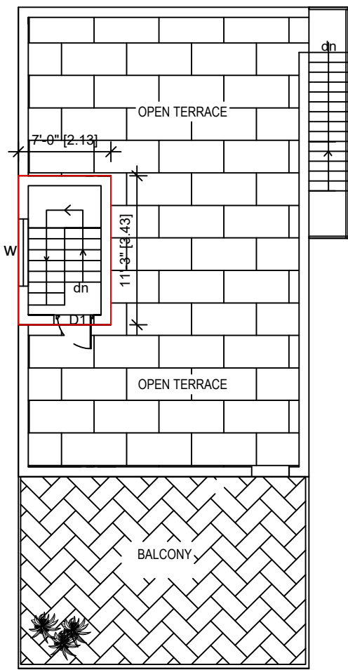
PRO. HEAD ROOM PLAN.
