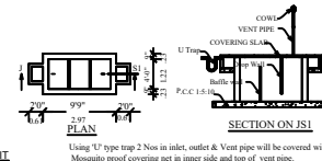
SEPTIC TANK DETAILS
