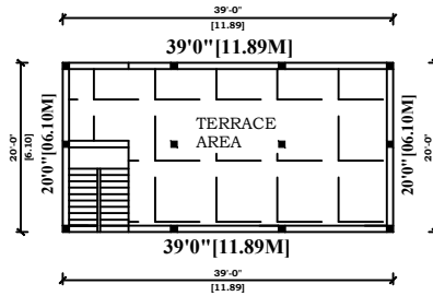
TERRACE FLOOR PLAN.
