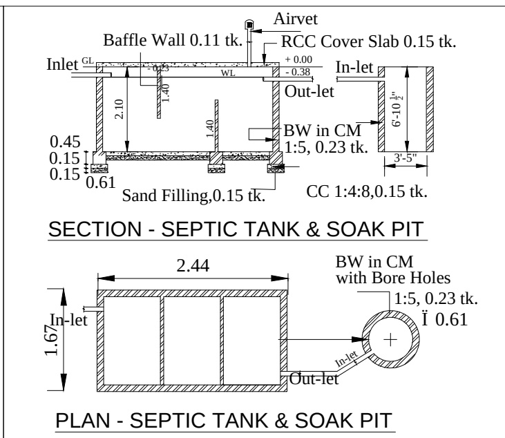
PLAN - SEPTIC TANK & SOAK PIT
