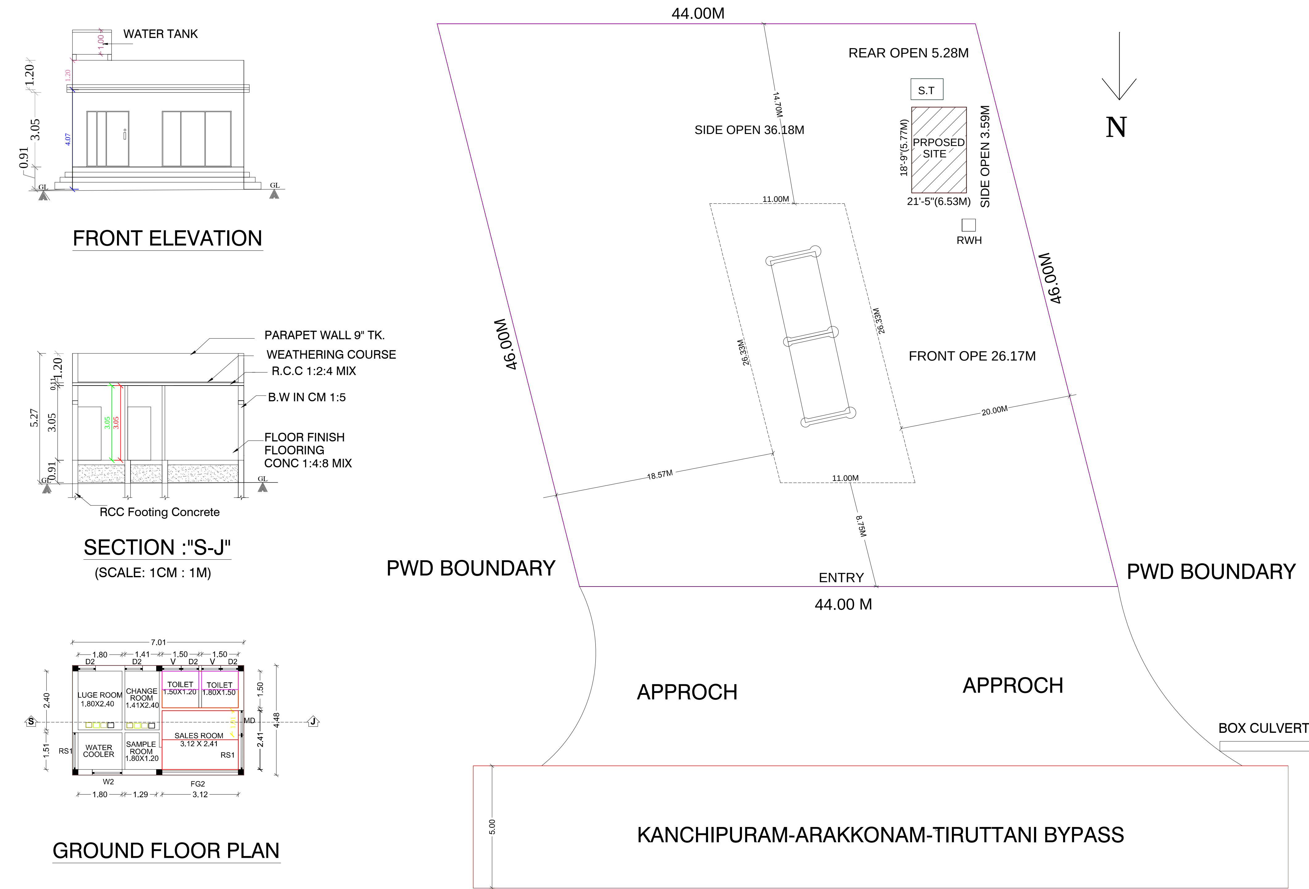
SITE PLAN
