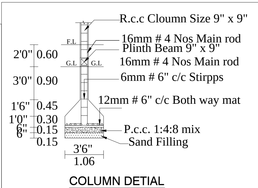
COLUMN DETAIL
