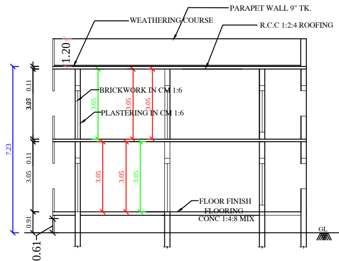
SECTION ON "J-J"
