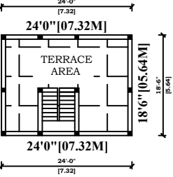
TERRACE FLOOR
