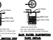
WATER HARVESTING TANK DETAIL
