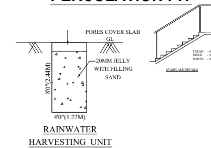
PERCULATION PIT
