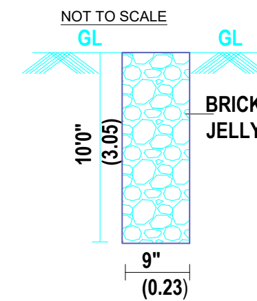
PERCULATION PIT
