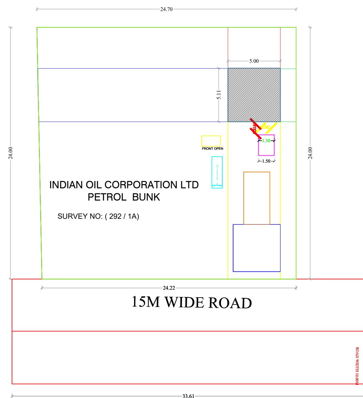
SITE PLAN
