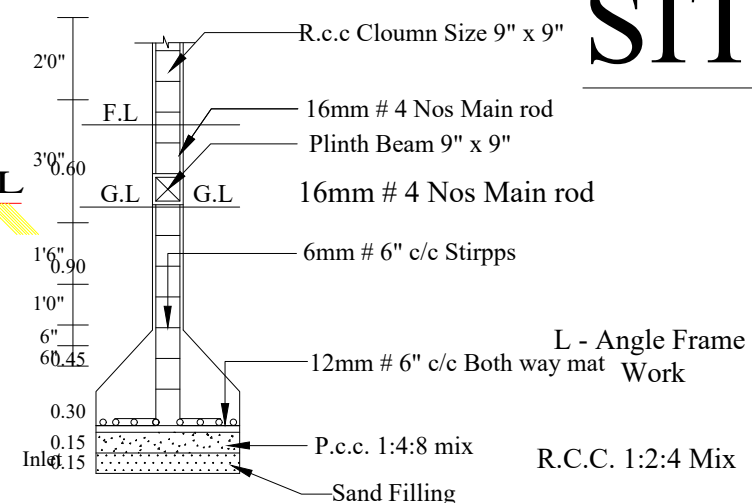
COLUMN DETIAL
