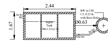
PLAN - SEPTIC TANK & SOAK PIT
