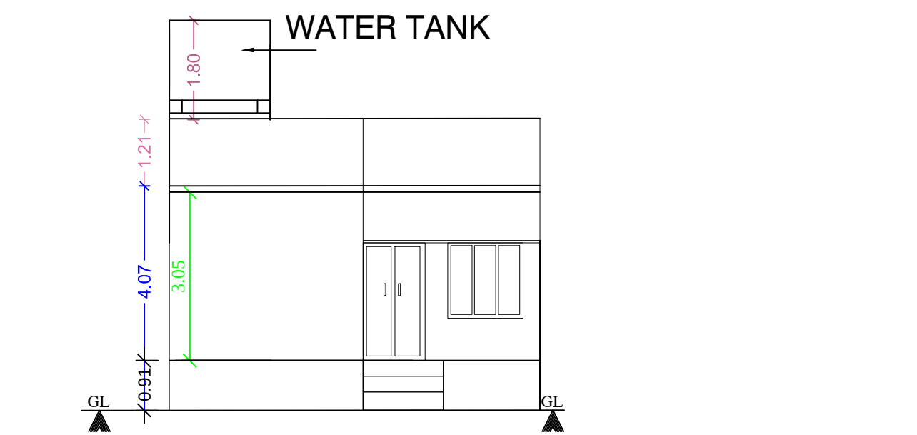
FRONT ELEVATION
