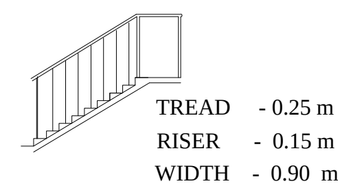
STAIRCASE DETAILS
