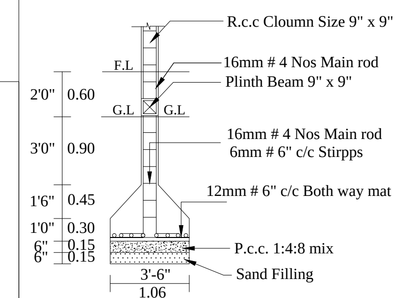
COLUMN DETIAL
