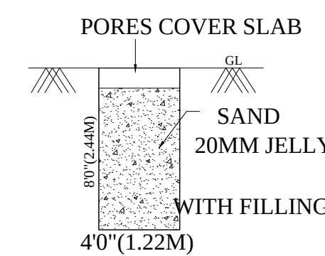
RAINWATER HARVESTING UNIT
