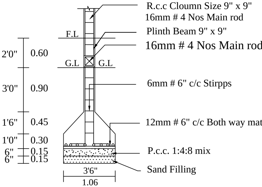
COLUMN DETIAL
