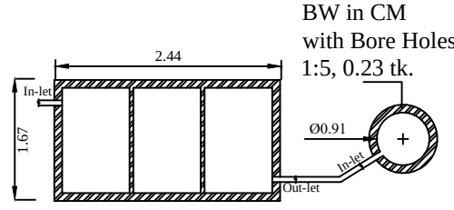
PLAN - SEPTIC TANK & SOAK PIT (1.98x1.21x2.10M)
