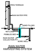
RAIN WATER HARVESTING SYSTEM
