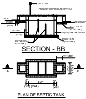
PLAN OF SEPTIC TANK
