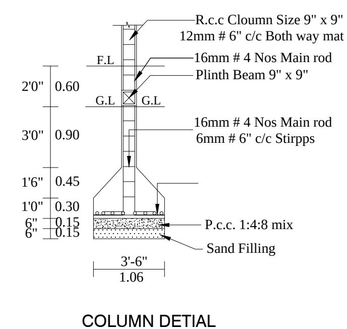
COLUMN DETIAL
