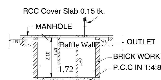
SECTION - SEPTIC TANK
