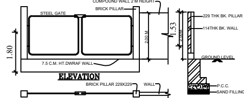
PLAN COMPOUND WALL DETAILS
