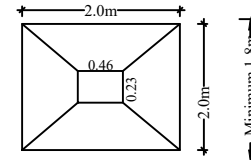
FOOTING / COLUMN DETAIL
