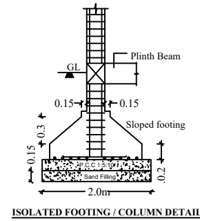
ISOLATED FOOTING / COLUMN DETAIL
