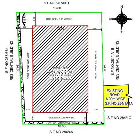
SITE PLAN SCALE- 1:200
