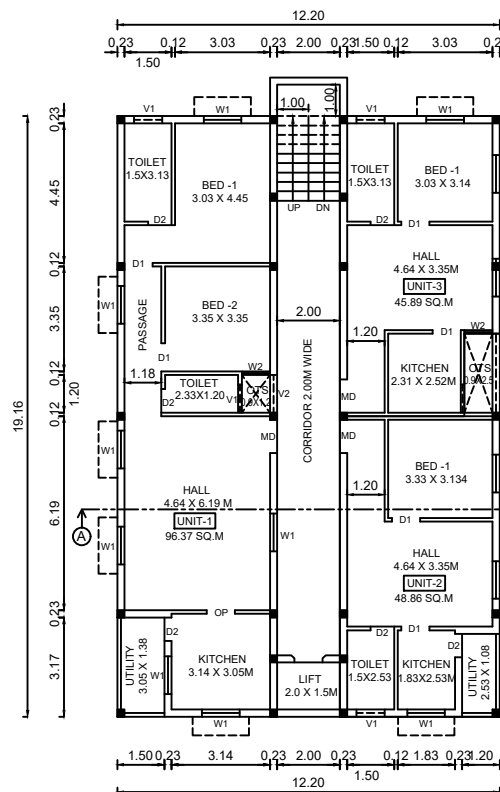
TYPICAL FLOOR PLAN [SECOND & THIRD]
