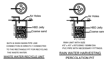
WASTE WATER RECYCLE UNIT
