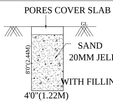
RAINWATER HARVESTING UNIT
