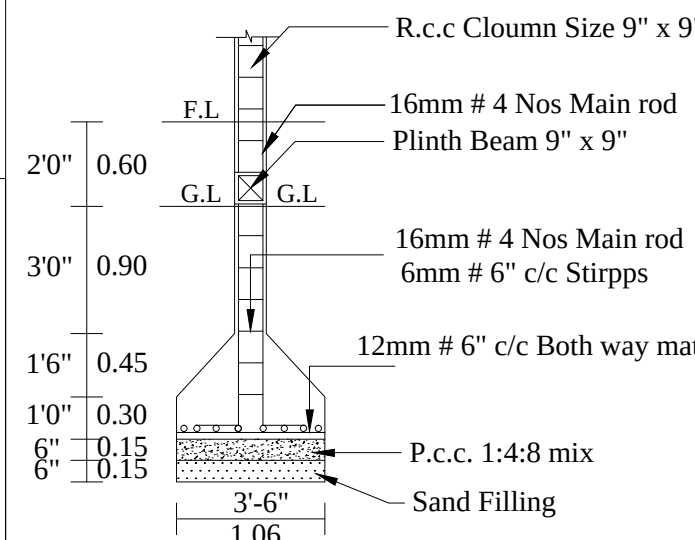
COLUMN DETIAL
