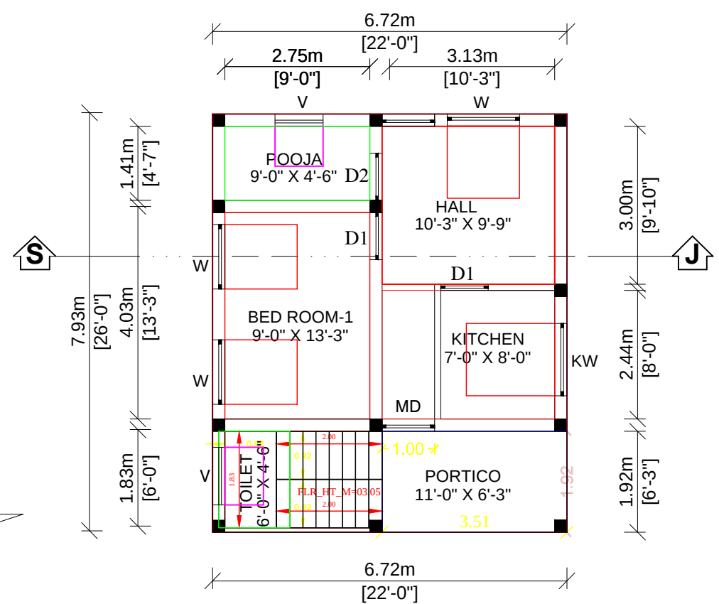
GROUND FLOOR AND HEAD ROOM PLAN
