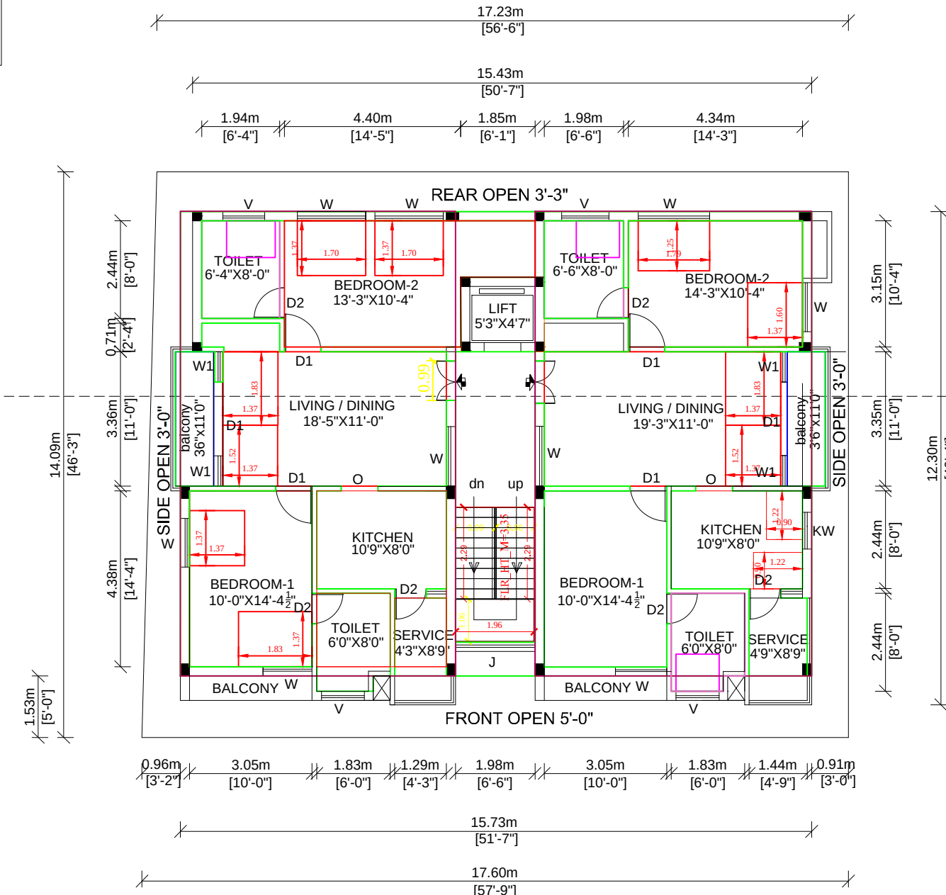
TYPICAL_FLOOR_PLAN=1,2,3 FIRST FLOOR PLAN (PROPOSED)
