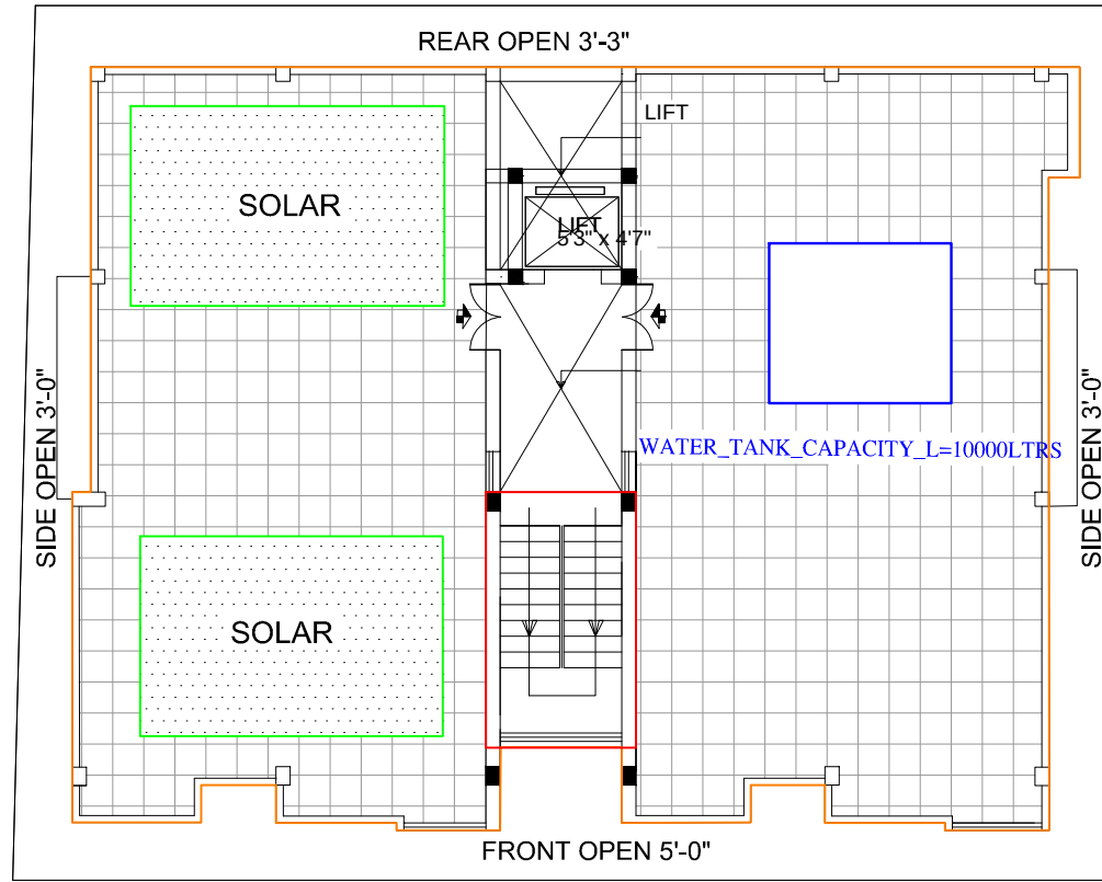
TERRACE FLOOR PLAN (PROPOSED)
