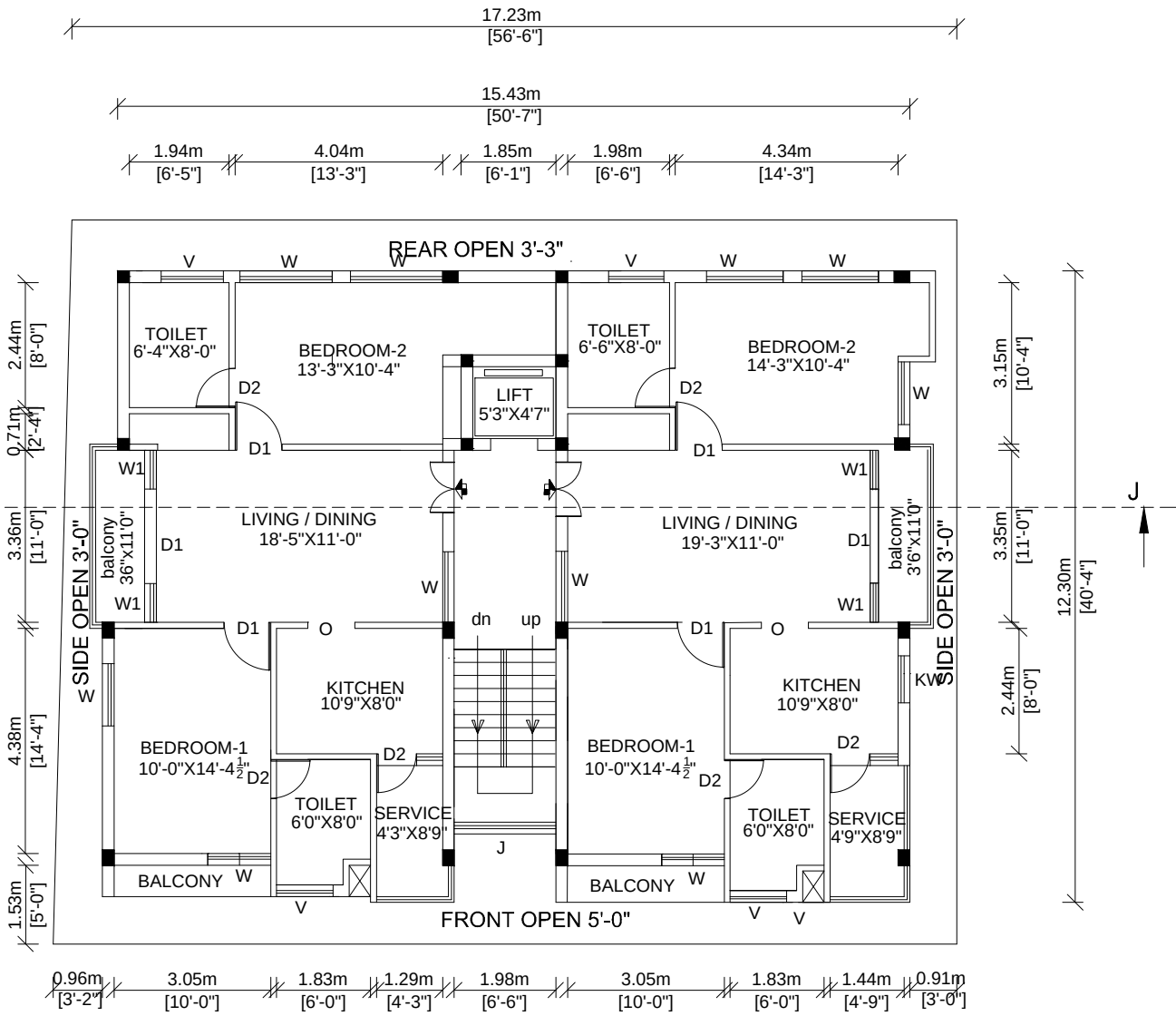
TYPICAL SECOND & THIRD FLOOR PLAN (PROPOSED)
