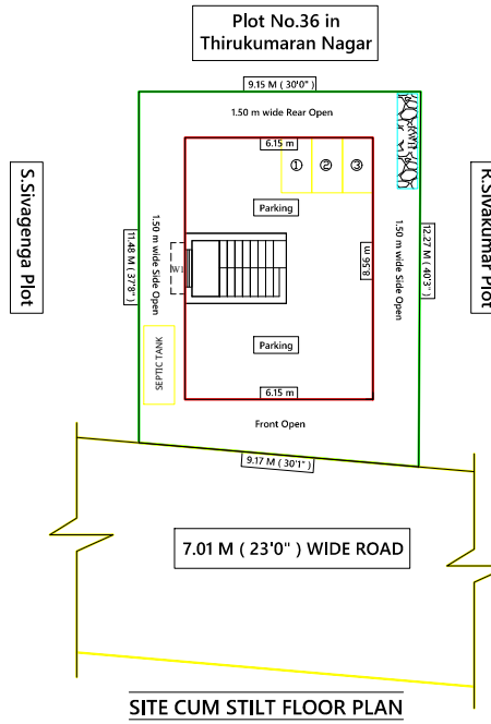
SITE CUM STILT FLOOR PLAN
