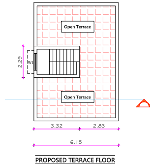
PROPOSED TERRACE FLOOR
