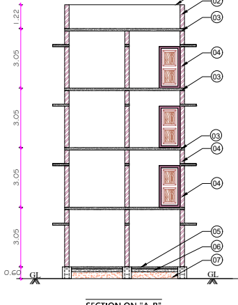
SECTION ON "A-B"
