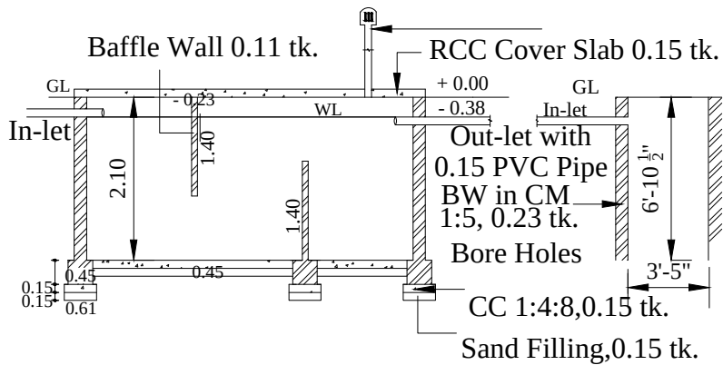
SEPTIC TANK & SOAK PIT
