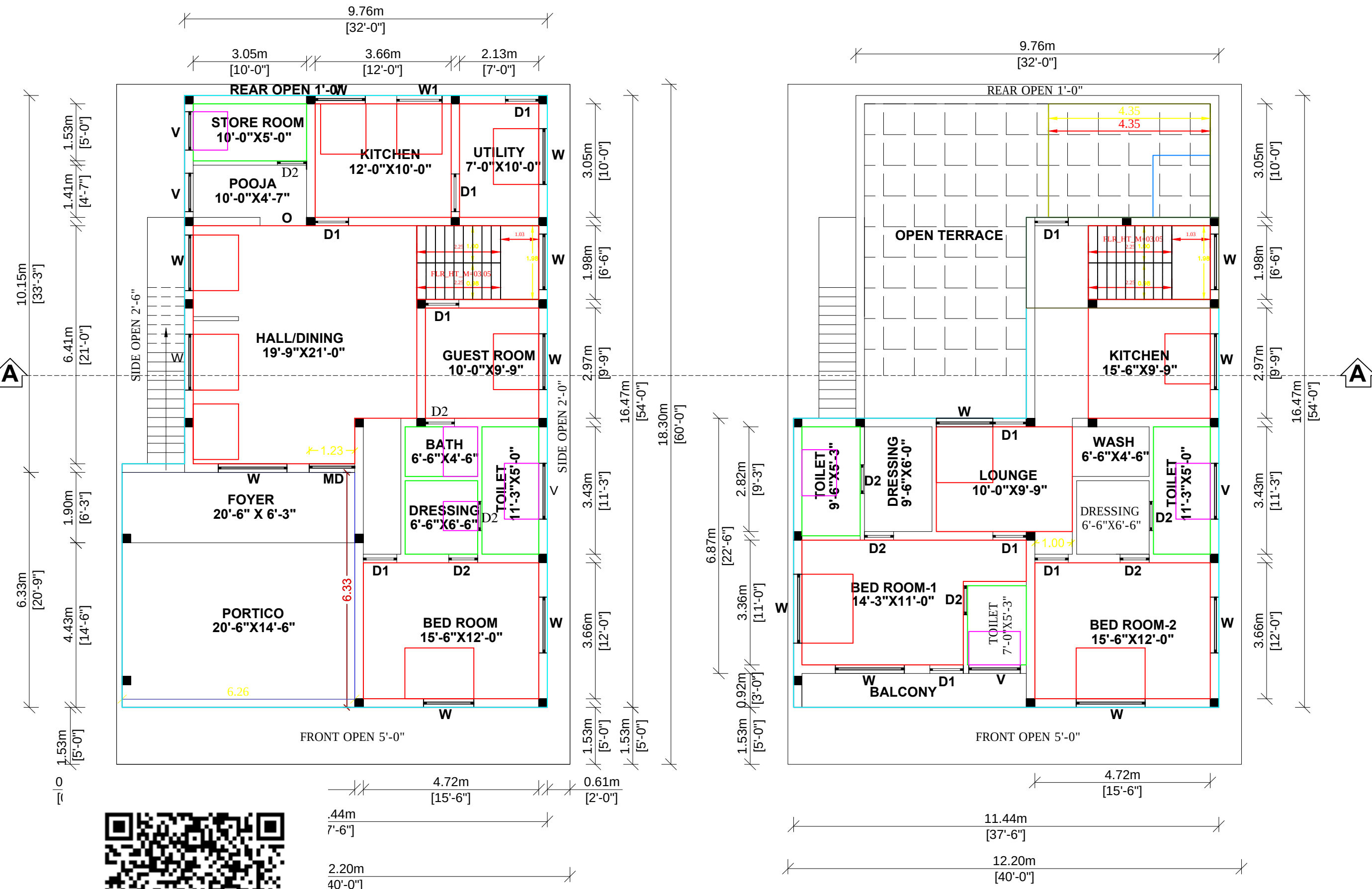
FLOOR PLAN
