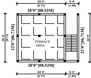
TERRACE FLOOR
