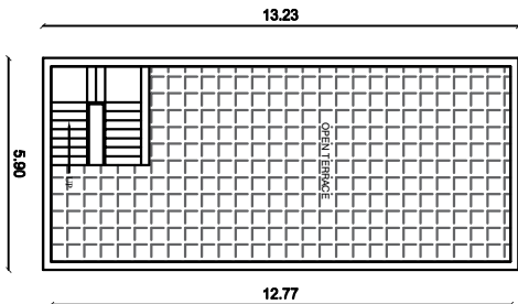
TERRACE FLOOR PLAN
