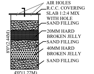
RAINWATER HARVESTING UNIT RW. - SIZE 4'0" X 4'0" X 10'0" - 3 NOS USING 150MM PIPE AND NECESSARY SPECIALS.
