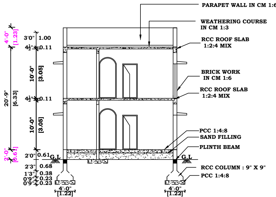
SECTION - KK
