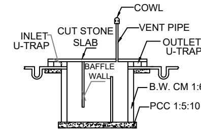
SEPTIC TANK DETAILS SIZE :6'0" x 3'0" x 6'0"
