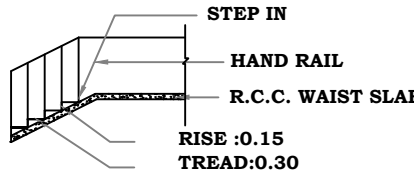
STAIR DETAILS
