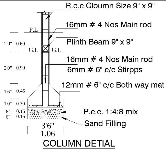
COLUMN DETIAL
