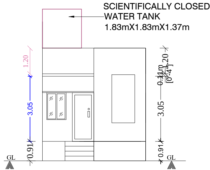
FRONT ELEVATION
