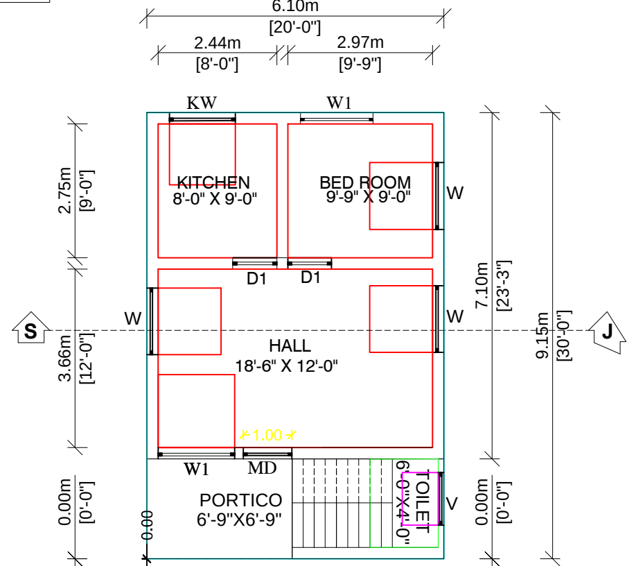
GROUND FLOOR PLAN-1
