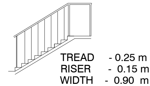
STAIRCASE DETAILS
