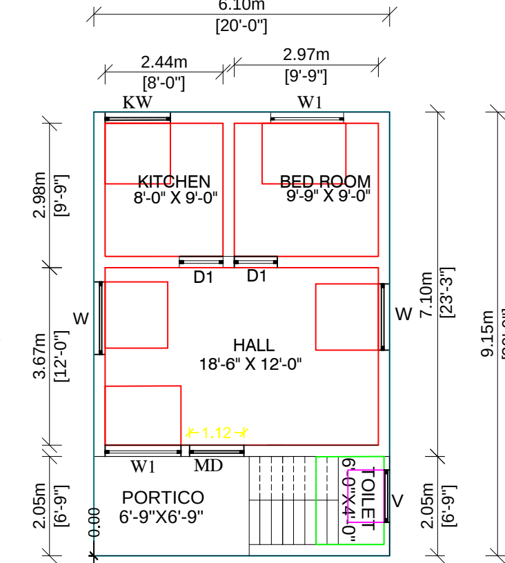
GROUND FLOOR PLAN-2
