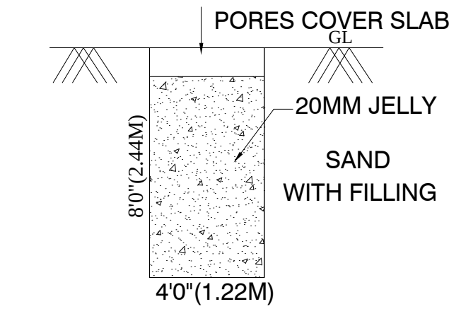
RAINWATER HARVESTING UNIT
