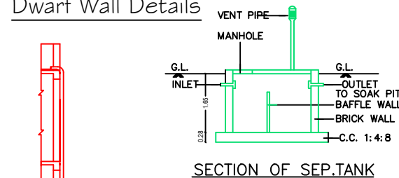
SECTION OF SEP.TANK
