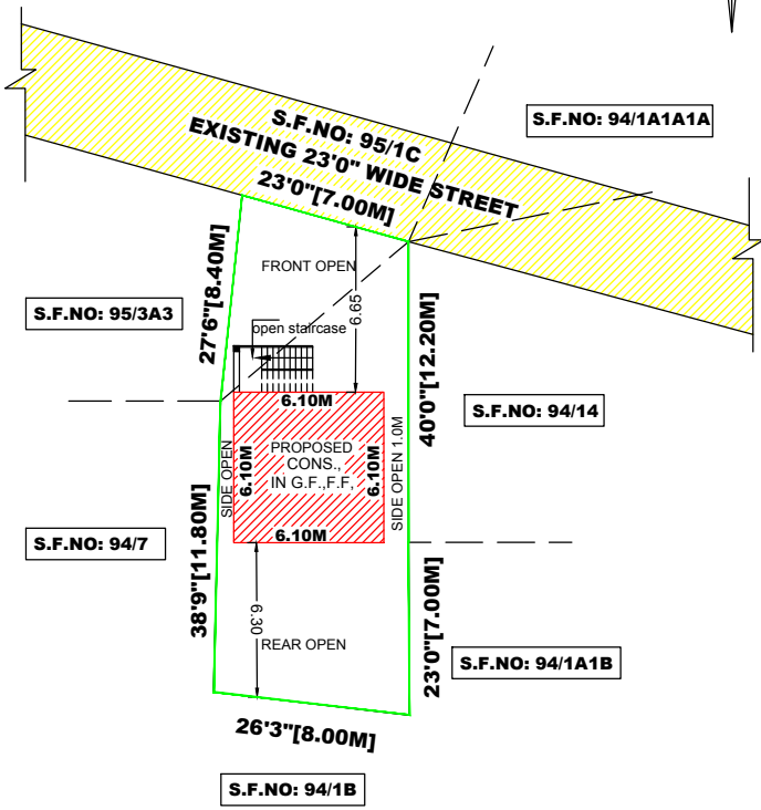
SITE PLAN
