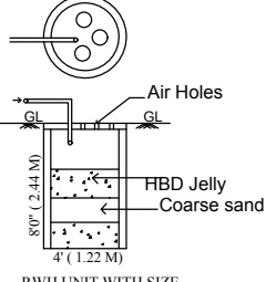
RAIN WATER HARVESTING TANK DETAIL
