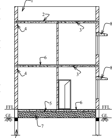
SECTION ON - "JS"
