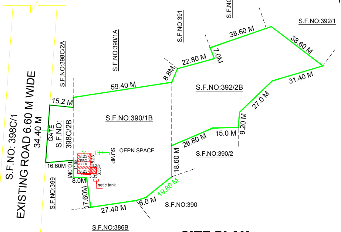
SITE PLAN
