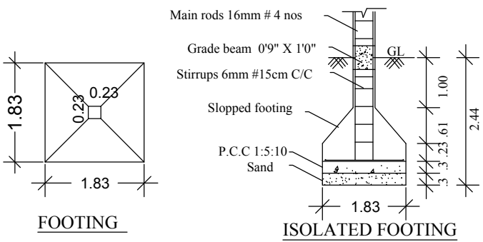
COLUMN DETAIL
