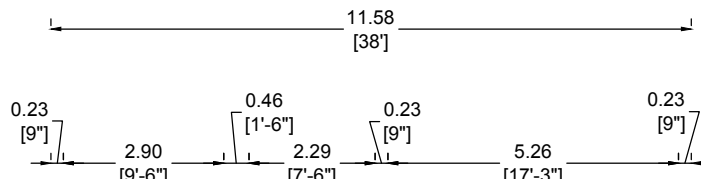
FRONT ELEVATION
