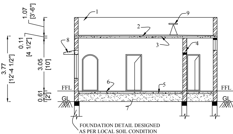
SECTION ON "JS"
