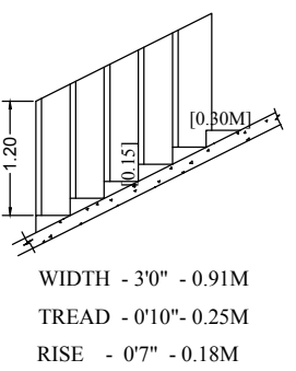
STAIRCASE DETAILS SCALE: 1INCH = 4FEET (OR) 1CM=0.50M
