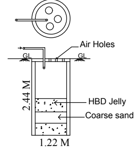
RAIN WATER HARVESTING TANK DETAIL
