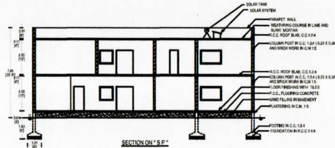
SECTION ON "S.P."
