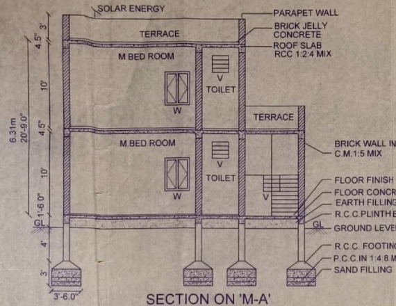
SECTION ON 'M-A'
