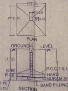
FOUNDATION DETAILS:
