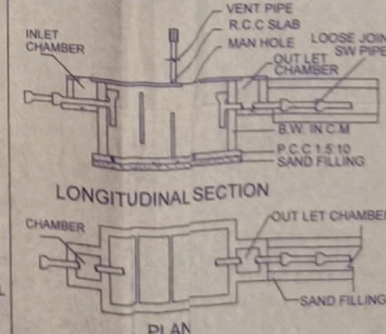
SEPTIC TANK:
