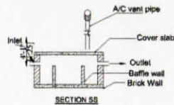
SECTION SS
