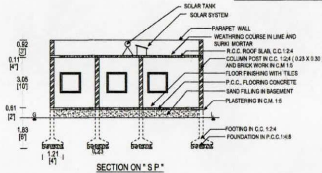
SECTION ON " S P "
