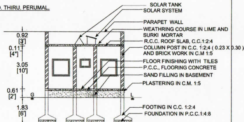
SECTION ON " S P "
