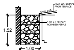
RAINWATER HARVESTING TRENCH
