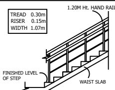
STAIRCASE DETAILS
