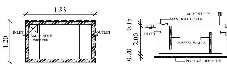
SEPTIC TANK DETAILS
