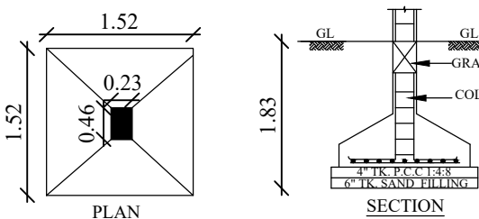
FOUNDATION DETAIL
