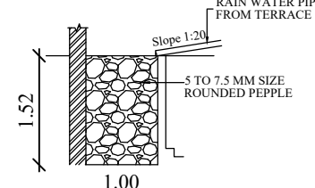
RAINWATER HARVESTING TRENCH
