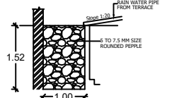
RAINWATER HARVESTING TRENCH
