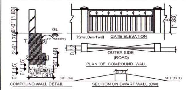
SECTION ON DWARF WALL (DW)
