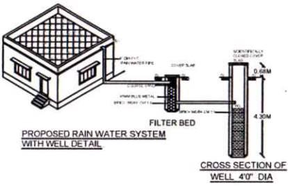
DETAILS OF COLLECTION PITS FOR RAIN WATER
