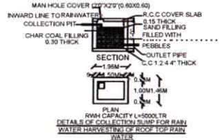
DETAILS OF COLLECTION PITS FOR RAIN WATER
