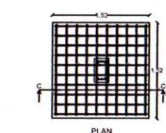
COLOUMN FOUNDATION DETAILS
