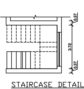
STAIRCASE DETAIL
