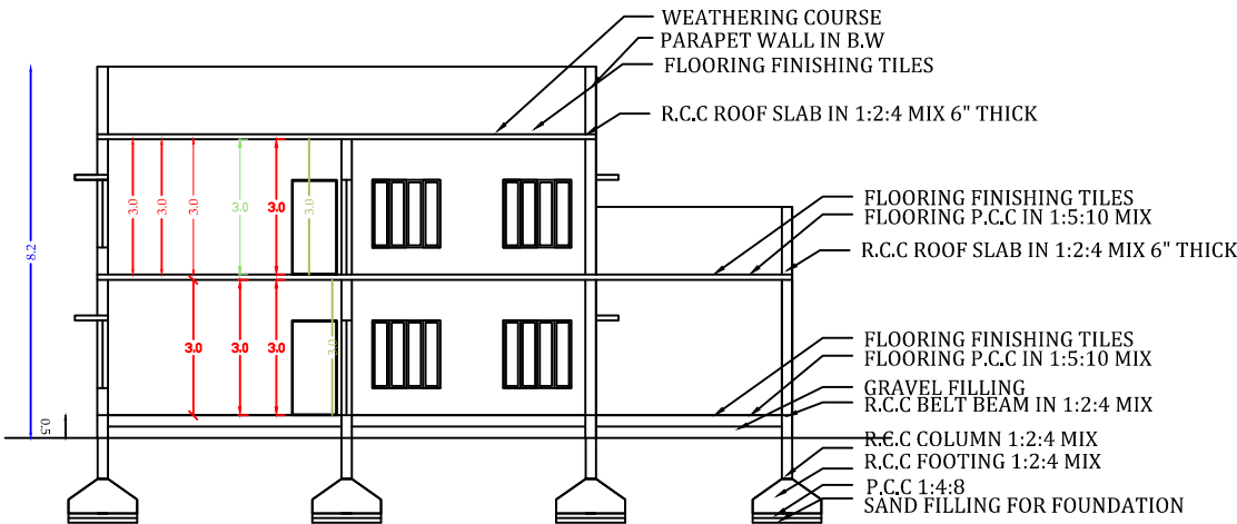
SECTION A TO B
