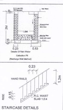
STAIRCASE DETAILS
