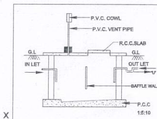
SEC. OF SEPTIC TANK
