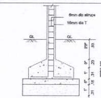
COLUMN FOUNDATION DETAIL
