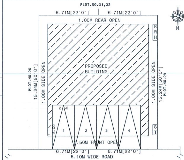
SITE PLAN SCALE: 1"=16'0" [1:200]
