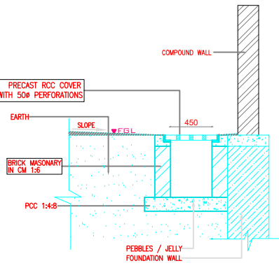
STORM WATER DRAIN DETAIL
