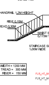
DETAILS OF STAIRCASE SCALE 1:50
