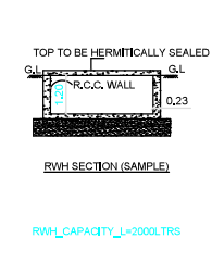
RAIN WATER COLLECTION PIT
