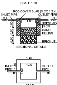
DETAILS OF ORGANIC FILTRATION BED SCALE 1:50
