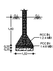
DETAILS OF RCC COLUMN SCALE 1:50
