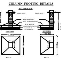
COLUMN FOOTING DETAILS
