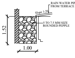
RAINWATER HARVESTING TRENCH
