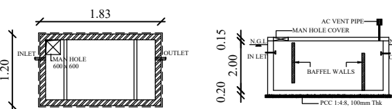
SEPTIC TANK DETAILS
