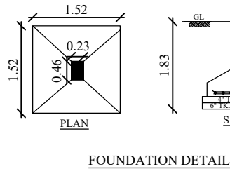
FOUNDATION DETAIL
