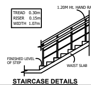
STAIRCASE DETAILS
