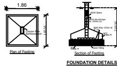
FOUNDATION DETAILS
