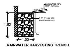
RAINWATER HARVESTING TRENCH
