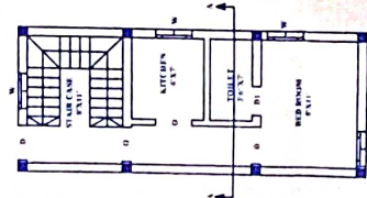
FIRST FLOOR PLAN - WEST FACING
