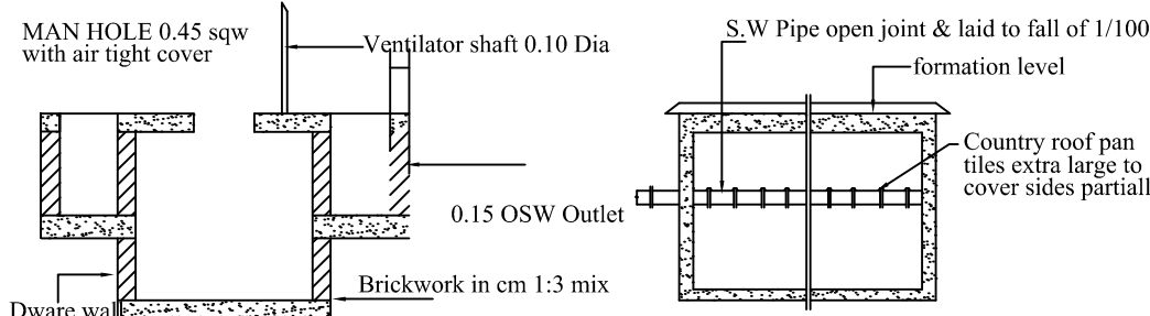
Section of Dispersion trench
