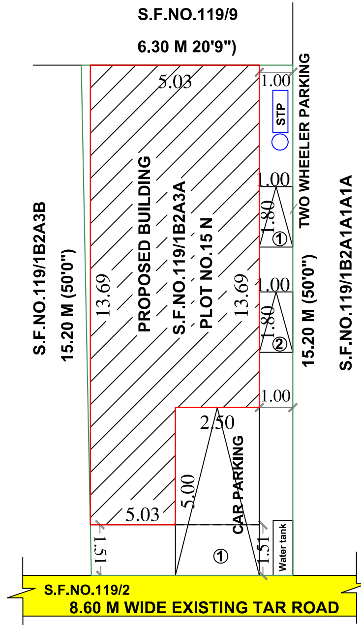
SITE PLAN
