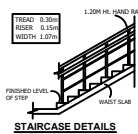
STAIRCASE DETAILS
