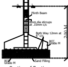
Section of Footing
