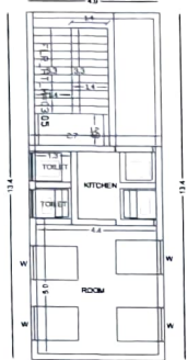
PLAN
